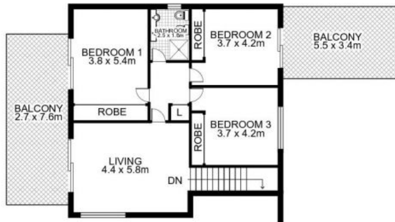
TOP FLOOR
